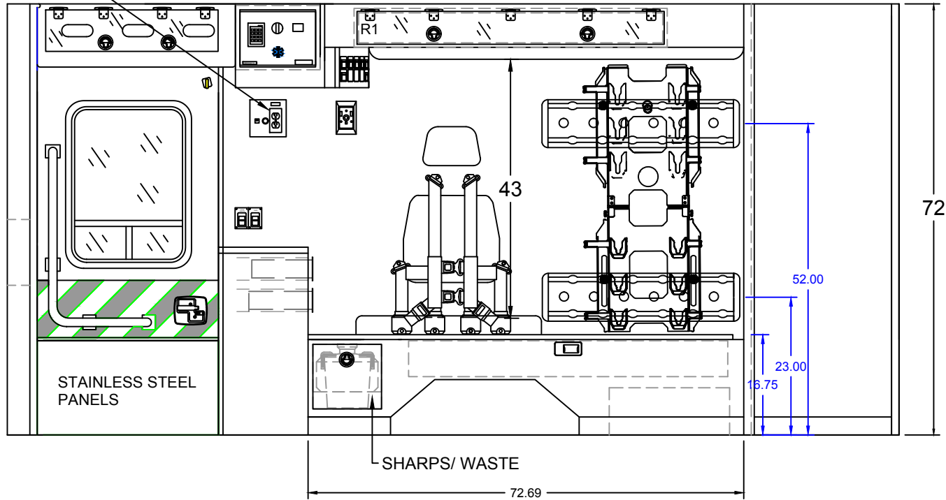
INTERIOR CABINET DIMENSIONS IN INCHES
