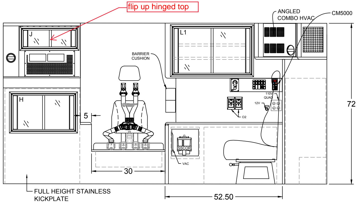
INTERIOR CABINET DIMENSIONS IN INCHES
