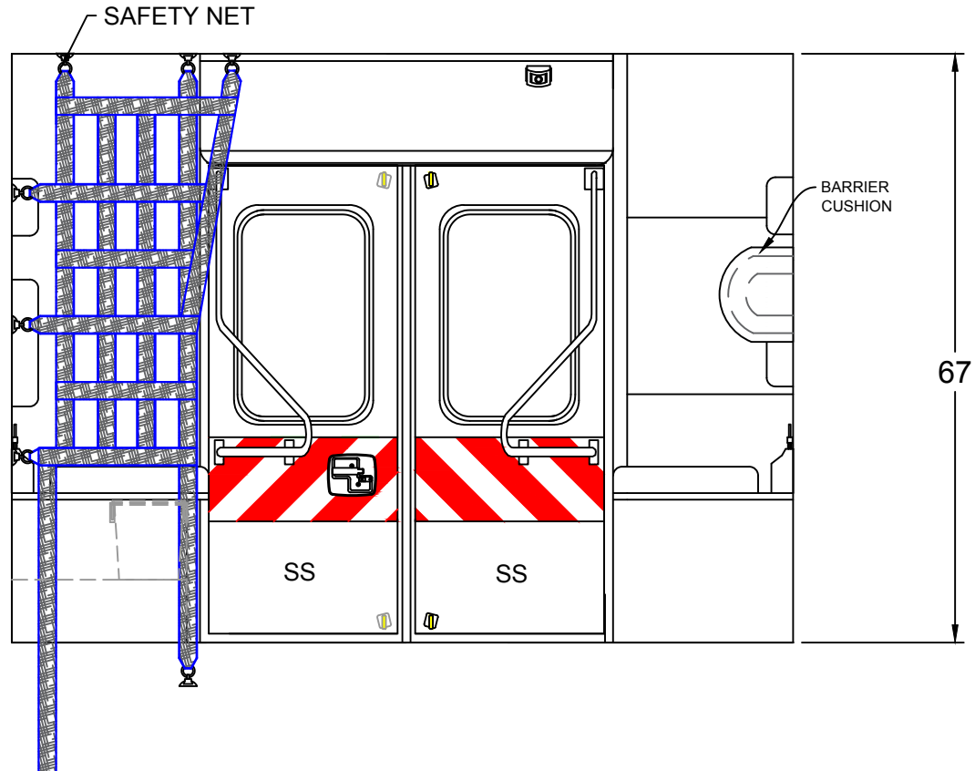
INTERIOR CABINET DIMENSIONS IN INCHES
