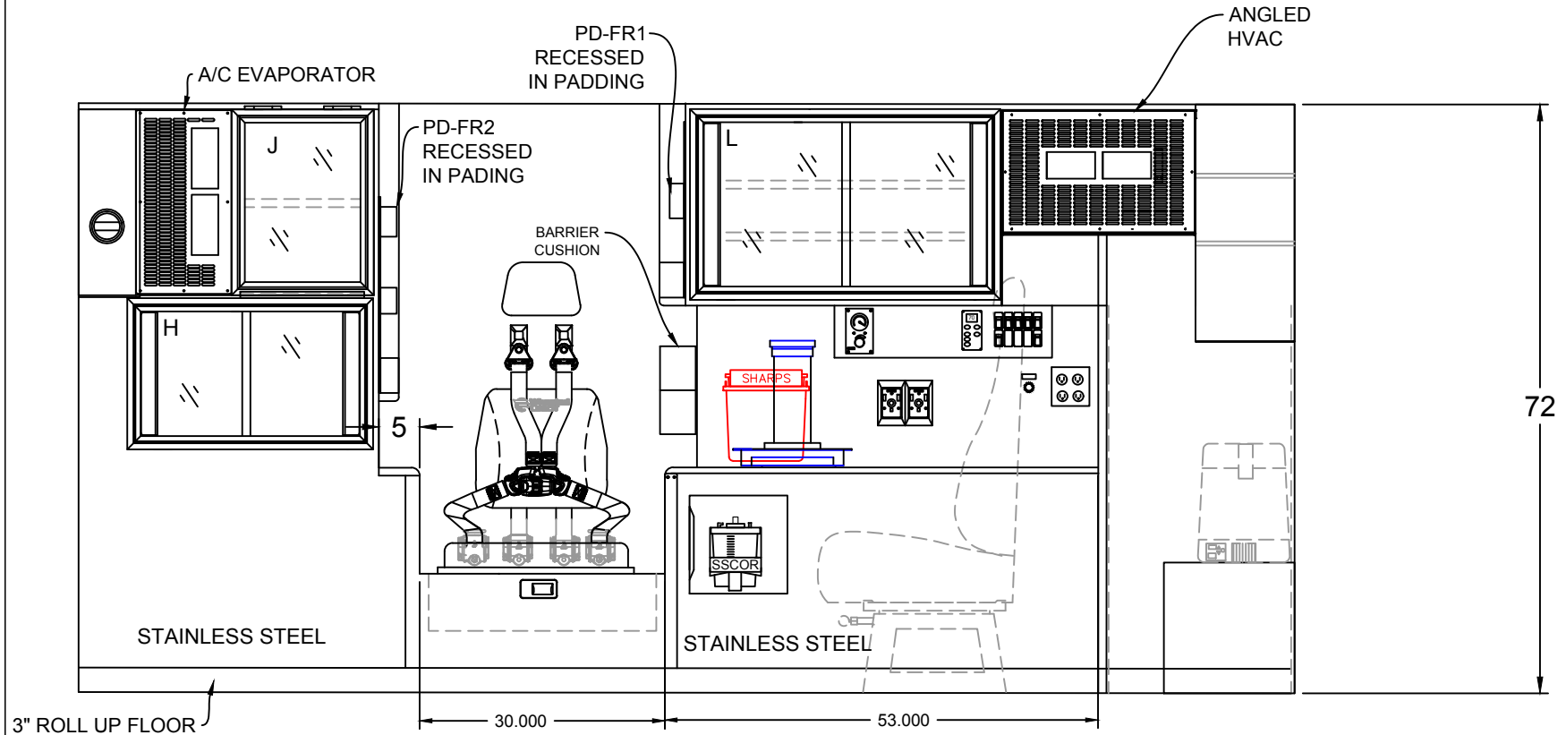
INTERIOR CABINET DIMENSIONS IN INCHES
